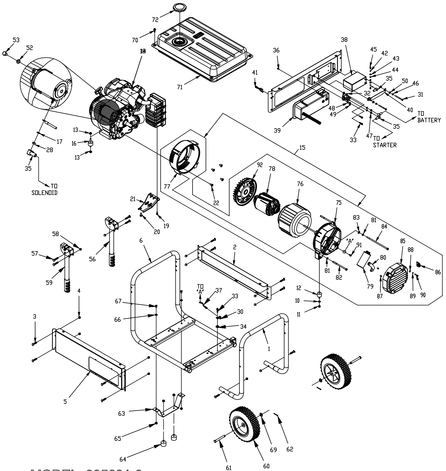
MODEL: 005681-0 GP 8000E ELEC START
