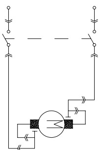
Electric circuit
